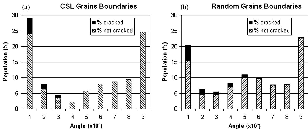
Fig. 11 Distribution of the orientations of (a) CSL type grain boundaries (b) random grain boundaries. The orientations are defined by the angle \alpha between the direction normal to the boundary plane and
