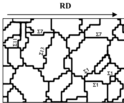
Fig. 5 OIM micrograph of the hot-dip galvanized zinc coating. Coincident boundaries ( \Sigma \leq 28 ) are selected according to the Brandon-type criterion (Eq. 1) with v_0 = 10^\circ . Non-labeled boundaries are random grain boundaries
