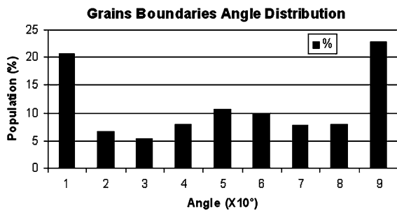
Fig. 10 Distribution of the grain boundary orientations according to the angle \alpha defined by the normal to the grain boundary plane and the direction of uniaxial tension
