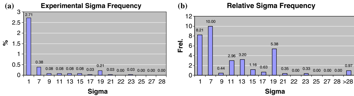
Fig. 7 (a) Experimental \Sigma -Frequency and (b) Relative \Sigma -Frequency scaled to random texture
